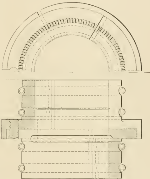
SELF ADJUSTING PISTON PACKING.
